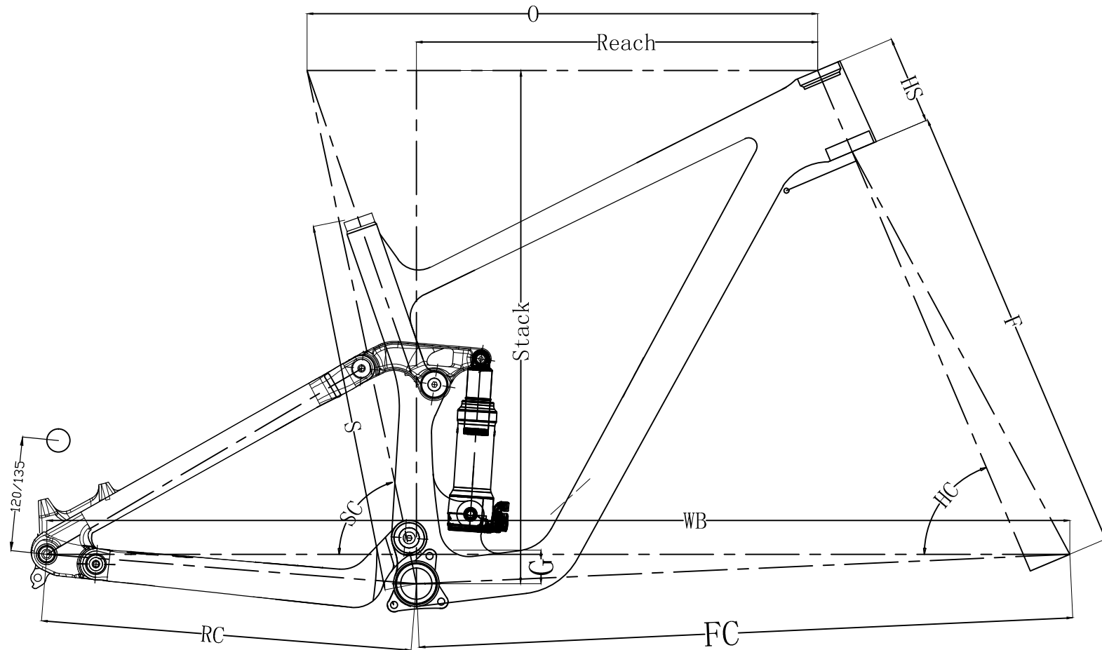
CFM-1001 Geometry
