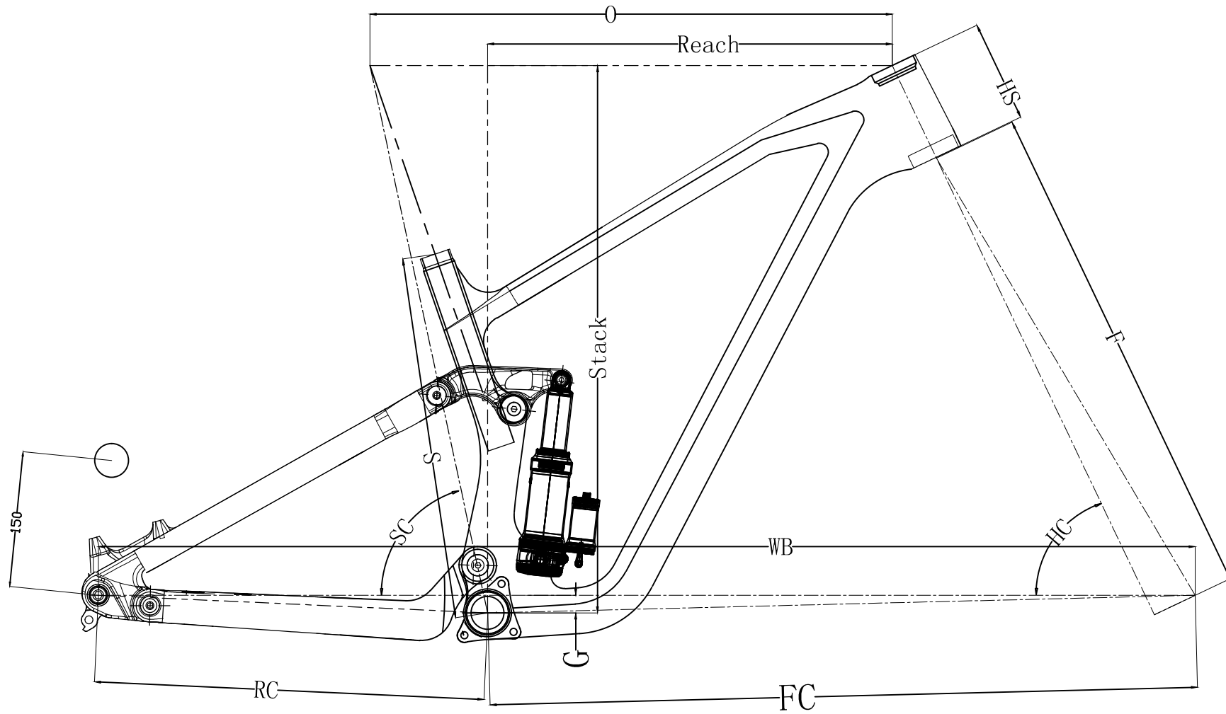
CFM-1002 Geometry
