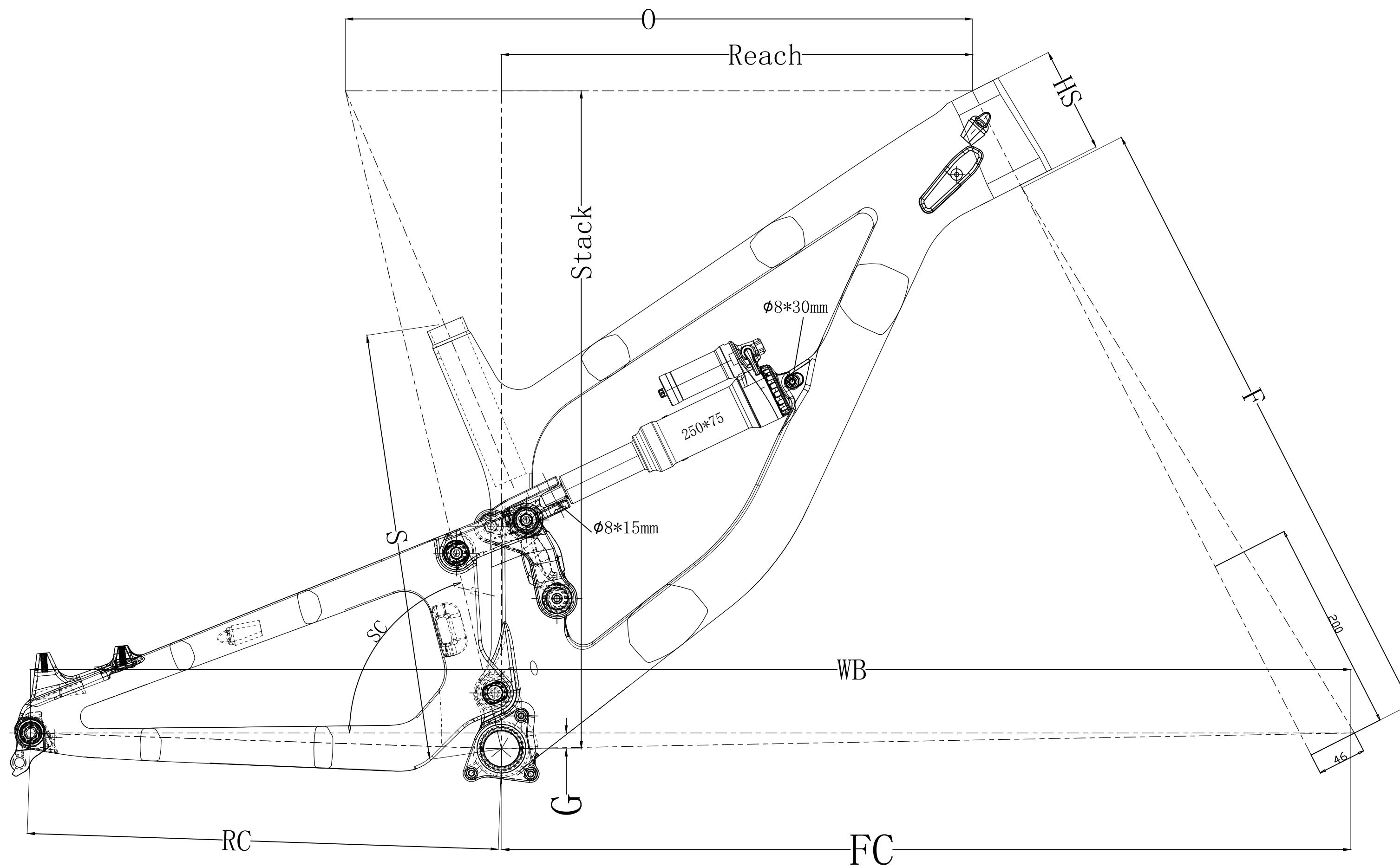
CFM-1286 Geometry
