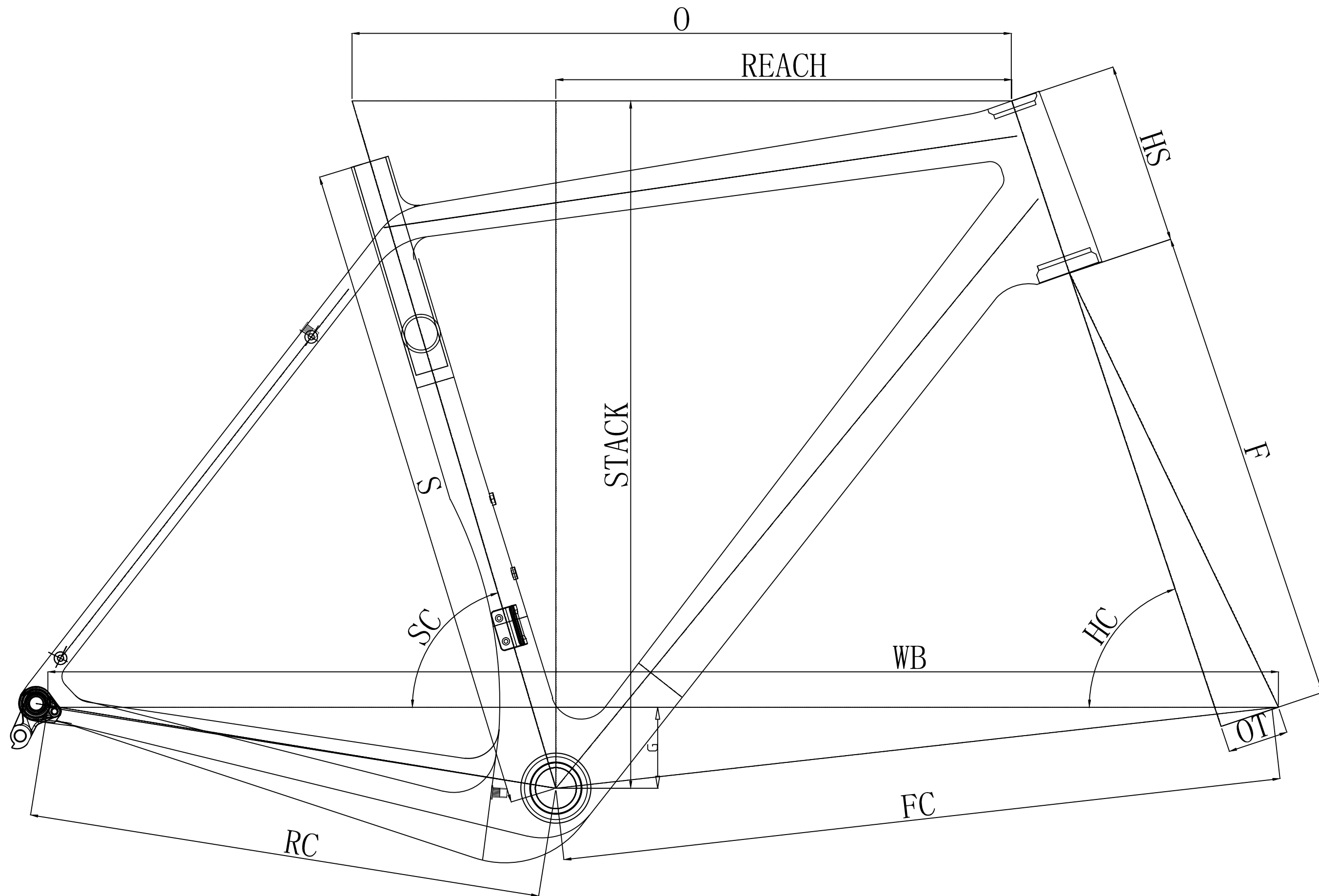
CFM-696 Geometry
